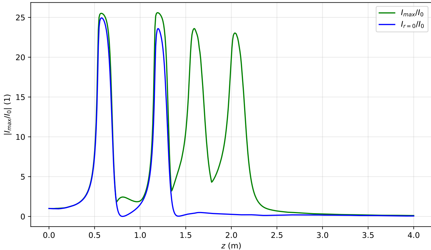
I_{max}(x=0, y=0, z)/I_0 , P_{in}=4.3P_{cr} , noisy input, artificial time
